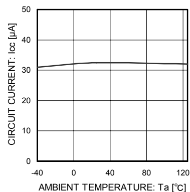
Fig. 12 Total Supply Current vs Temperature
