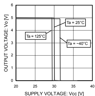
Fig. 6 Overvoltage Protection
