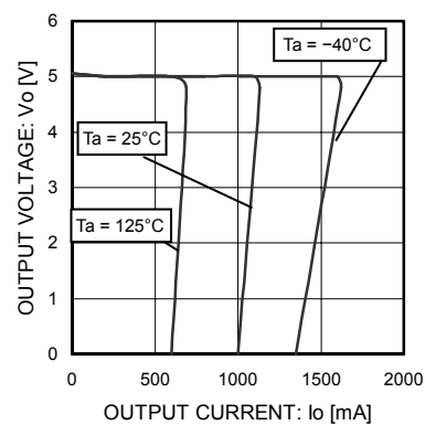
Fig. 3 Output Voltage vs Load
